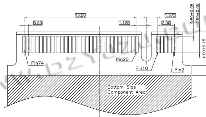
RECOMMENDED MOULD FINGER LAYOUT DEFAULT TOLERANCE±0.05
